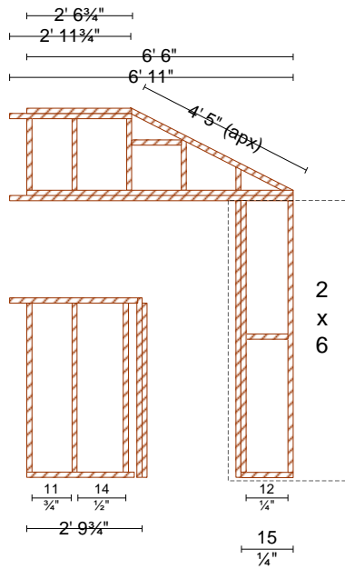
2x4 wall (with 2x6 section)
