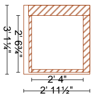
Corner Cap, 2x4 & plywood
