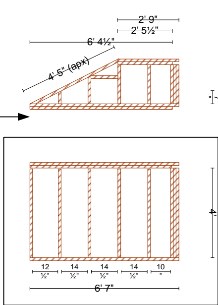
2x6 wet wall
